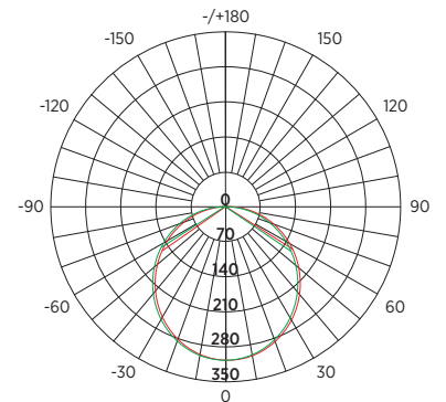
AVERAGE BEAM ANGLE (50%): 112.5 DEG
